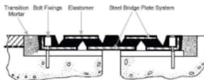
Typical cross section through the fitted joint
